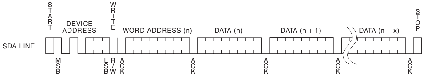
Figure 9. Page Write
