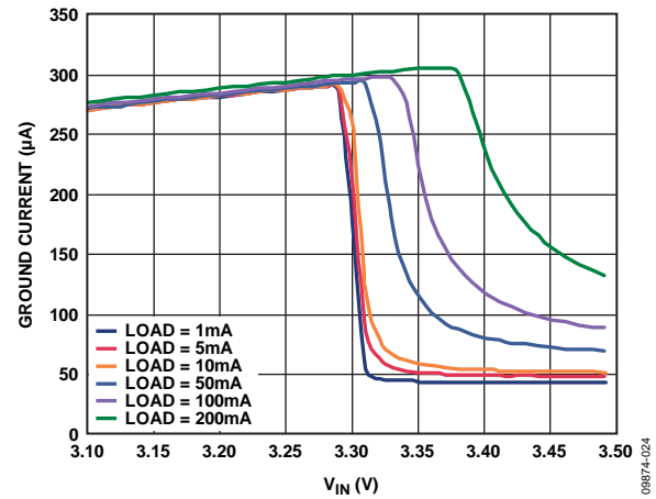
Figure 24. Ground Current vs. Input Voltage (in Dropout), V_{OUT1} = 3.3 \text{ V} , V_{RIPPLE} = 50 \text{ mV} , C_{OUT} = 1 \mu\text{F}
