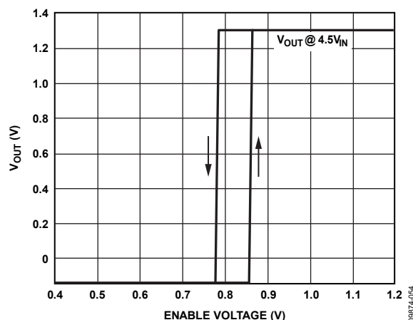
Figure 50. Typical ENx Pin Operation
