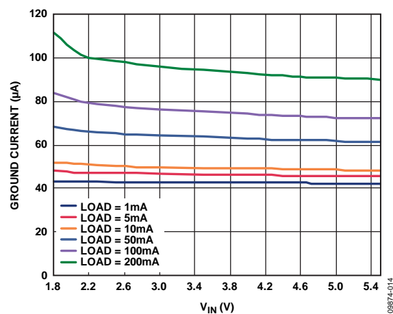
Figure 14. Ground Current vs. Input Voltage, Single Output Loaded, V_{\text{RIPPLE}} = 50 \text{ mV} , C_{\text{OUT}} = 1 \mu\text{F}
