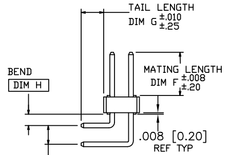
END VIEW
