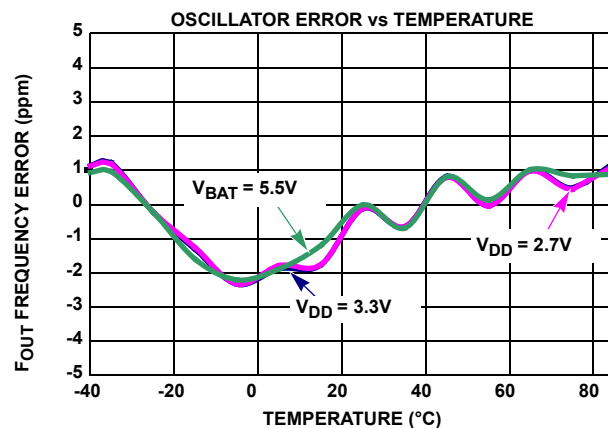
FIGURE 2. PERFORMANCE CURVE
