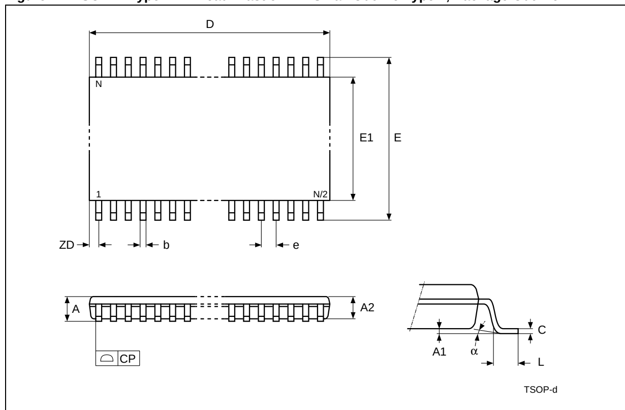
Figure 14. TSOP44 Type II - 44 lead Plastic Thin Small Outline Type II, Package Outline
