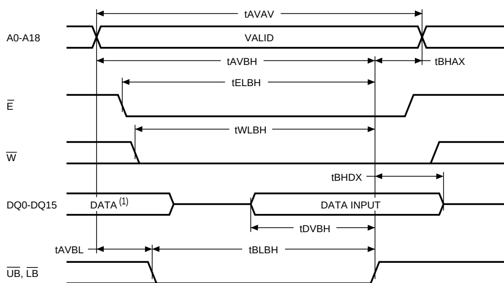
Figure 12. \overline{\text{UB}}/\overline{\text{LB}} Controlled, Write AC Waveforms
