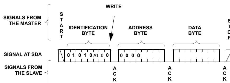
FIGURE 23. BYTE WRITE SEQUENCE
