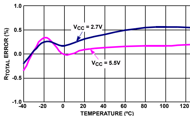
FIGURE 8. R_{\text{TOTAL}} ERROR vs TEMPERATURE FOR 10kΩ (W)
