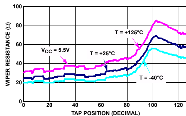
FIGURE 20. WIPER RESISTANCE vs TAP POSITION WHEN PRECISION IS OFF
