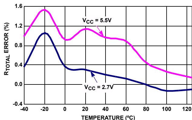
FIGURE 7. R_{\text{TOTAL}} ERROR vs TEMPERATURE FOR 100kΩ (T)
