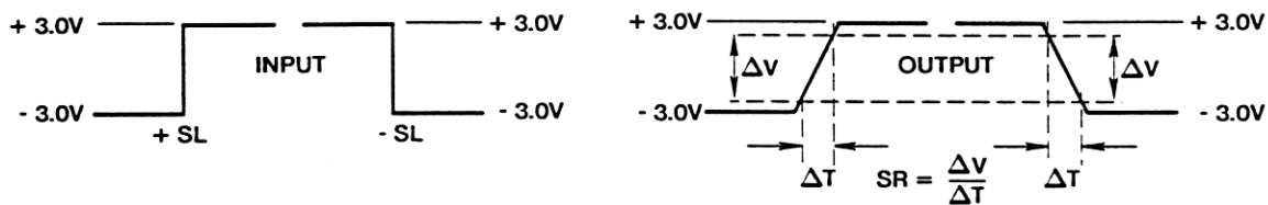
SLEW RATE WAVEFORMS
