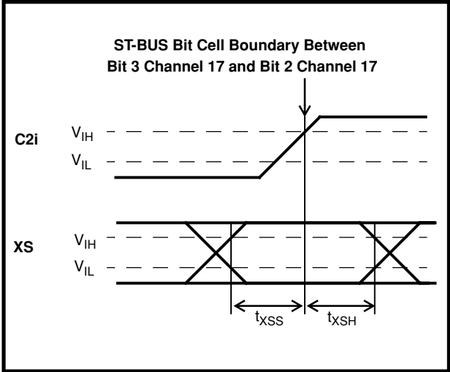
Figure 23 - XS Timing
