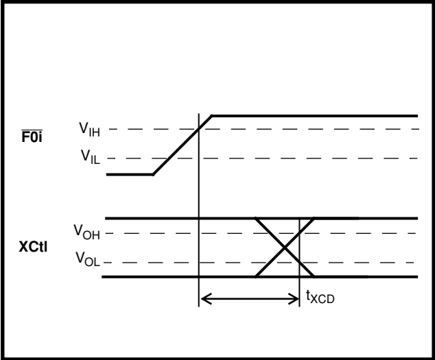
Figure 22 - XCtl Timing
