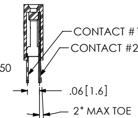
SECTION "B"-"B" BCS-1XX-X-S-DE
