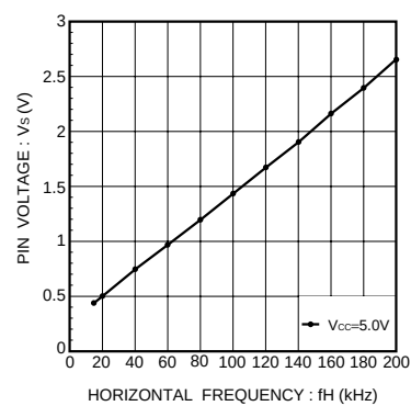
Fig.8 VSEPA horizontal frequency vs. pin voltage
