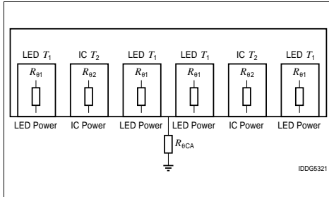
Thermal Model
