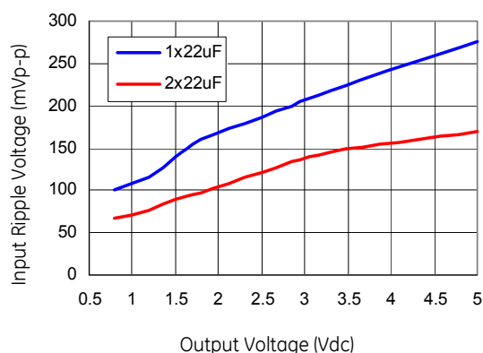
Figure 40. Input ripple voltage for various output voltages with 1x22 μF or 2x22 μF ceramic capacitors at the input (12A load). Input voltage is 12V.
