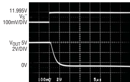
Step Response V_{SENSE} = 100\text{mV to } 5\text{mV}
