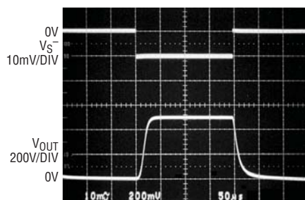
Step Response V_{SENSE} = 0\text{V to } 10\text{mV}, C_L = 1000\text{pF}, V_S^+ = 0\text{V}
