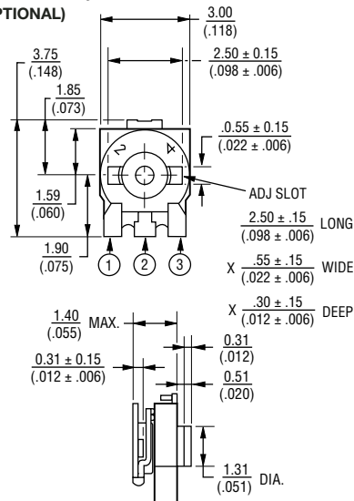
3303C,D-1 3-Terminal Both Sides Adjust (OPTIONAL)
