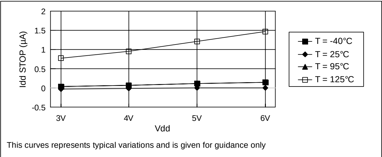
Figure 39. Idd STOP versus VDD for ROM devices
