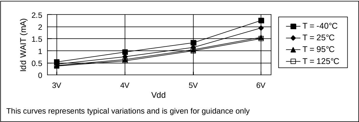
Figure 38. Idd STOP versus VDD for OTP devices
