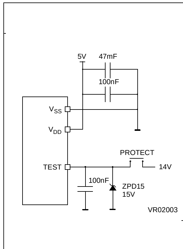
Figure 2. Programming Circuit
