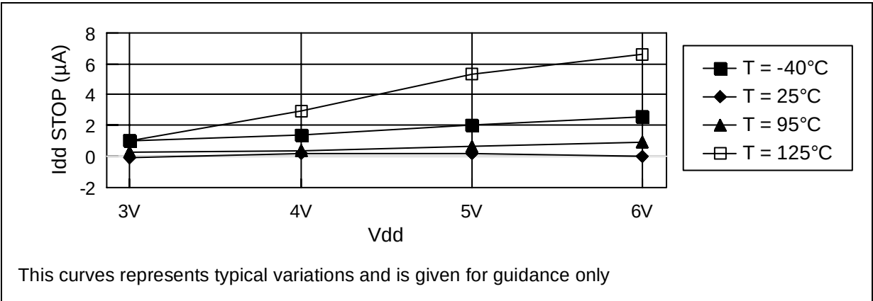
Figure 39. Idd STOP versus VDD for ROM devices
