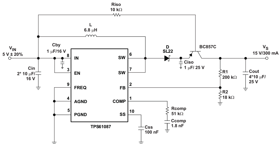
Figure 16. Typical Application with External Load Disconnect Switch
