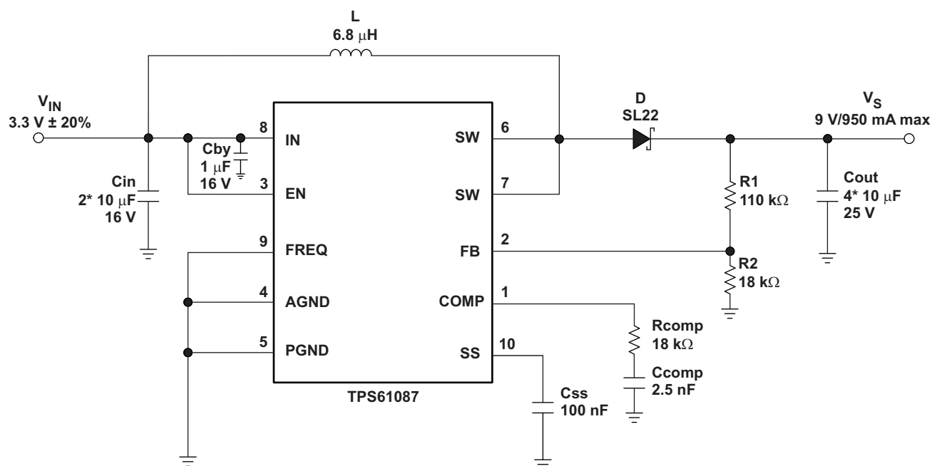
Figure 15. Typical Application, 3.3 V to 9 V ( f_{sw} = 650 kHz)
