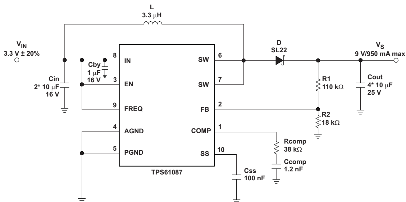
Figure 14. Typical Application, 3.3 V to 9 V ( f_{sw} = 1.2 MHz)
