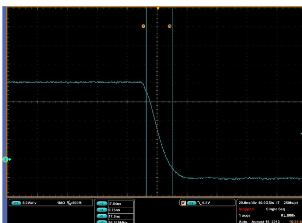
Figure 9. UCC27532DBV Input vs. Output PWM Fall Time
