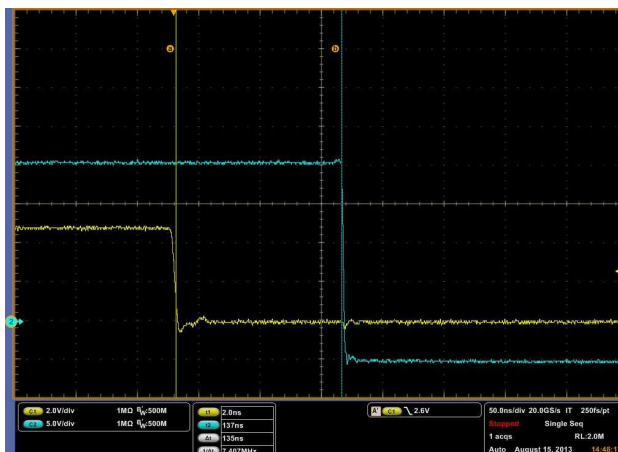
Figure 7. UCC27532DBV Input vs. Output PWM Propagation Delay (Low)
