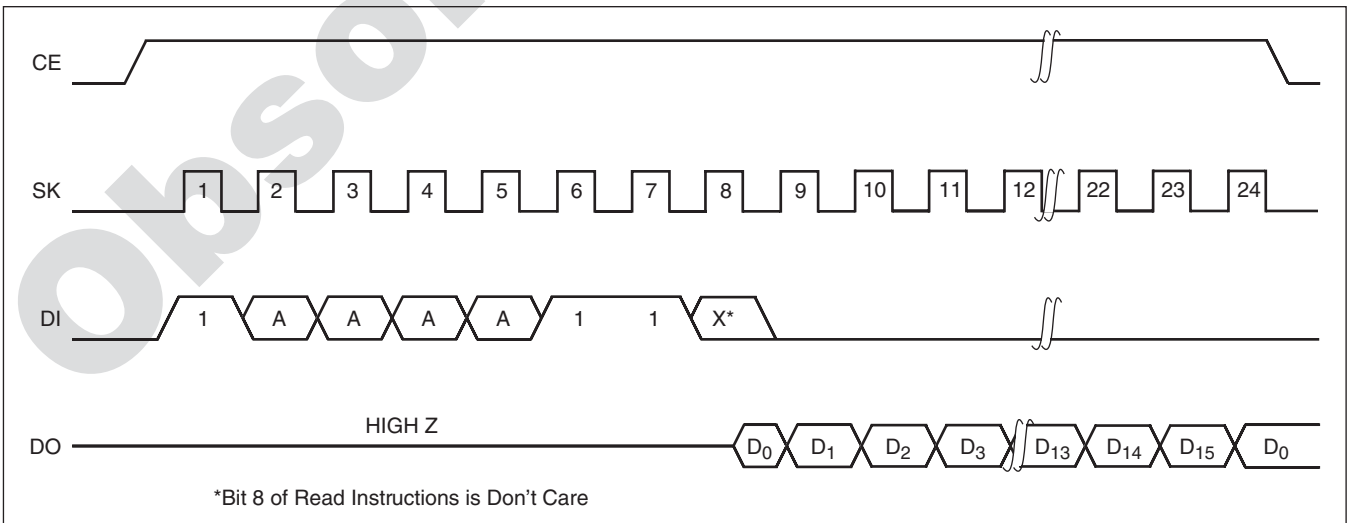
Figure 1. RAM Read
