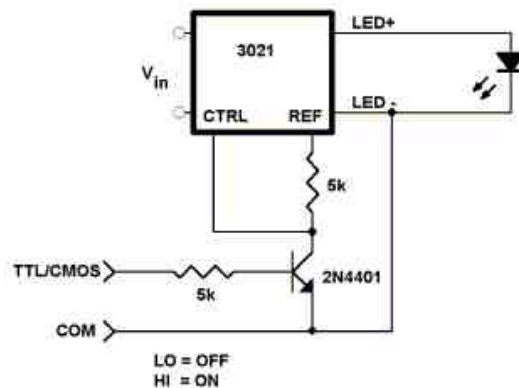
Figure 14. Pulse/Strobe input 5V=ON
