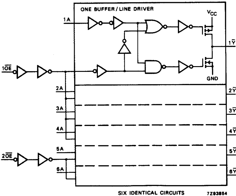
Fig.5 Logic diagram.
