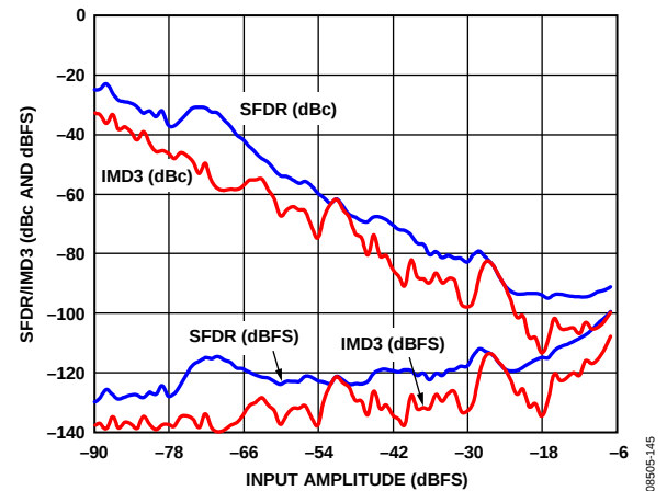
Figure 45. AD9255-125 Two-Tone SFDR/IMD3 vs. Input Amplitude ( A_{IN} ) with f_{IN1} = 169.1\text{ MHz} , f_{IN2} = 172.1\text{ MHz} , f_S = 125\text{ MSPS}
