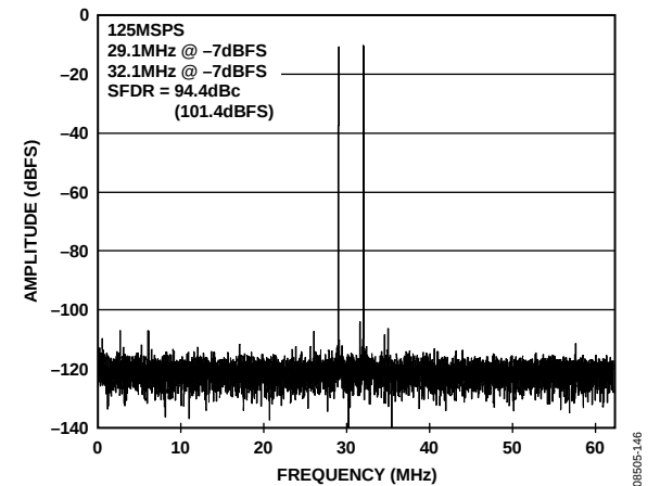
Figure 46. AD9255-125 Two-Tone FFT with f_{IN1} = 29.1\text{ MHz} and f_{IN2} = 32.1\text{ MHz}
