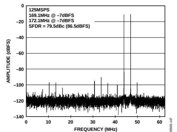
Figure 47. AD9255-125 Two-Tone FFT with f_{IN1} = 169.1\text{ MHz} and f_{IN2} = 172.1\text{ MHz}
