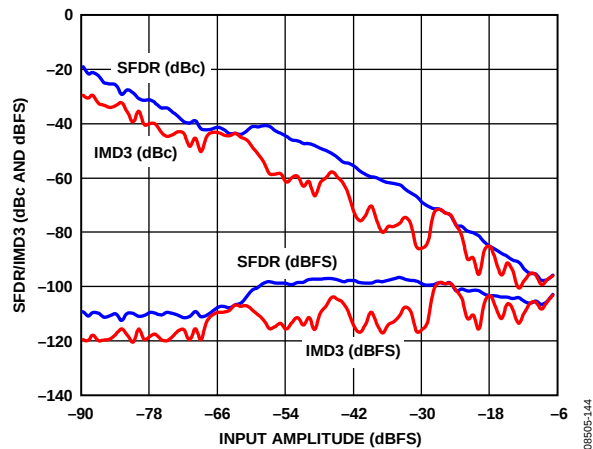
Figure 44. AD9255-125 Two-Tone SFDR/IMD3 vs. Input Amplitude ( A_{IN} ) with f_{IN1} = 29.1\text{ MHz} , f_{IN2} = 32.1\text{ MHz} , f_S = 125\text{ MSPS}
