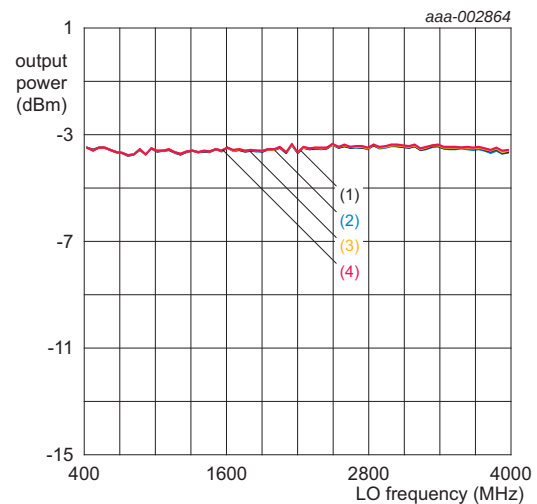
Fig 8. P_o versus f_{lo} and V_{CC}
