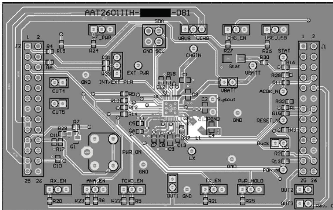
Figure 11: AAT2601/AAT2601A Evaluation Kit Top Layer.
