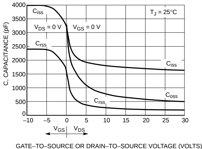
Figure 7. Capacitance Variation
