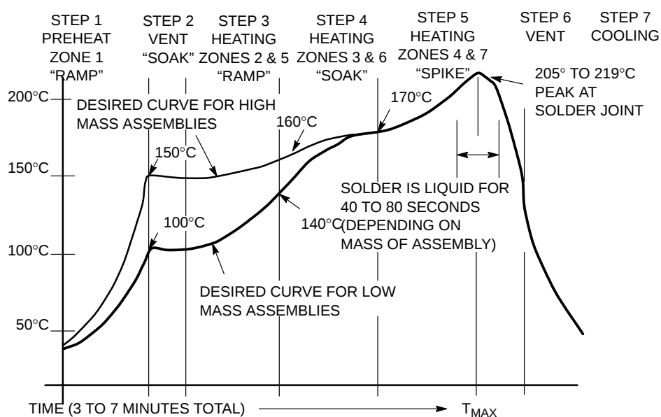
Figure 18. Typical Solder Heating Profile
