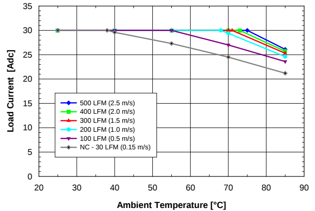
Fig. 1.8V.2: Available load current vs. ambient air temperature and airflow rates for SQE48T30018 converter mounted horizontally with air flowing from pin 3 to pin 1, MOSFET temperature \leq 120 °C, V_{in} = 48 V.
