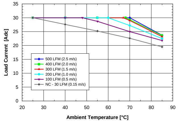
Fig. 2.5V.2: Available load current vs. ambient air temperature and airflow rates for SQE48T30025 converter mounted horizontally with air flowing from pin 3 to pin 1, MOSFET temperature \leq 120 °C, V_{in} = 48 V.
