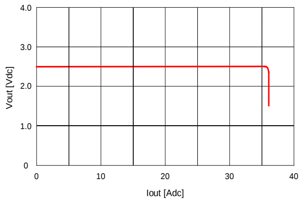
Fig. 2.5V.15: Output voltage vs. load current showing current limit point and converter shutdown point. Input voltage has almost no effect on current limit characteristic.
