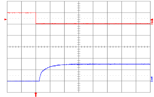
Fig. 1.5V.8: Turn-on transient at full rated load current (resistive) plus 10,000 \mu\text{F} at V_{in} = 48\text{ V} , triggered via ON/OFF pin. Top trace: ON/OFF signal (5 V/div.). Bottom trace: Output voltage (1 V/div.). Time scale: 2 ms/div.
