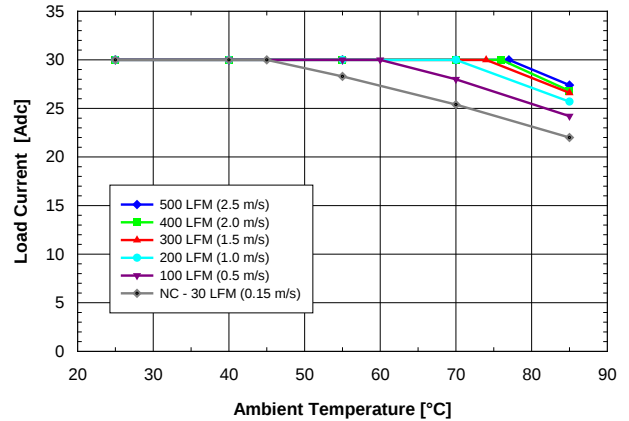
Fig. 1.5V.2: Available load current vs. ambient air temperature and airflow rates for SQE48T30015 converter mounted horizontally with air flowing from pin 3 to pin 1, MOSFET temperature \leq 120 °C, V_{in} = 48 V.
