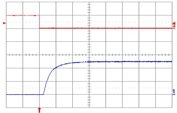
Fig. 2.5V.8: Turn-on transient at full rated load current (resistive) plus 10,000 \mu\text{F} at V_{in} = 48\text{ V} , triggered via ON/OFF pin. Top trace: ON/OFF signal (5 V/div.). Bottom trace: Output voltage (1 V/div.). Time scale: 2 ms/div.
