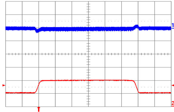
Fig. 1.2V.9: Output voltage response to load current step-change (10 A – 20 A – 10 A) at V_{in} = 48 V. Top trace: output voltage (100 mV/div.). Bottom trace: load current (10 A/div.). Current slew rate: 0.1 A/ \mu s. C_o = 1 \mu F ceramic. Time scale: 0.2 ms/div.
