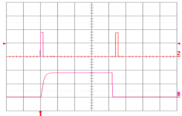
Fig. 2.5V.16: Load current (top trace, 20 A/div., 50 ms/div.) into a 10 m \Omega short circuit during restart, at V_{in} = 48 V. Bottom trace (20 A/div., 2 ms/div.) is an expansion of the on-time portion of the top trace.
