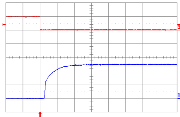
Fig. 2.5V.7: Turn-on transient at full rated load current (resistive) with no output capacitor at V_{in} = 48\text{ V} , triggered via ON/OFF pin. Top trace: ON/OFF signal (5 V/div.). Bottom trace: Output voltage (1 V/div.). Time scale: 2 ms/div.
