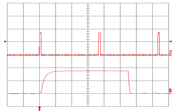
Fig. 3.3V.16: Load current (top trace, 20 A/div., 50 ms/div.) into a 10 \text{ m}\Omega short circuit during restart, at V_{in} = 48 \text{ V} . Bottom trace (20 A/div., 1 ms/div.) is an expansion of the on-time portion of the top trace.
