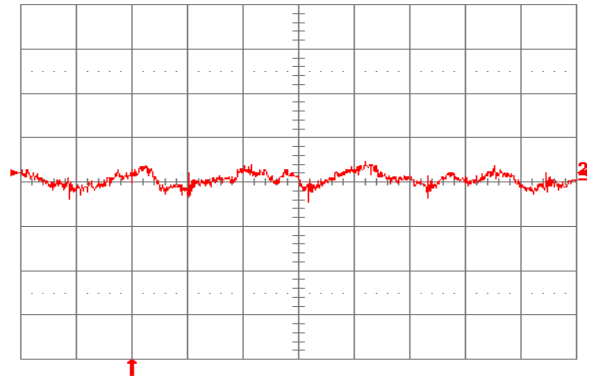
Fig. 2.5V.14: Input reflected-ripple current, i_s (10 mA/div.), measured through 10 \mu H at the source at full rated load current and V_{in} = 48 V. Refer to Fig. 2.5V.12 for test setup. Time scale: 1 \mu s/div.
