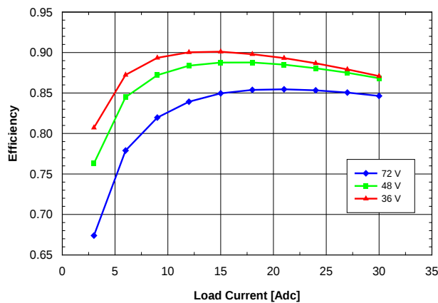
Fig. 1.8V.3: Efficiency vs. load current and input voltage for SQE48T30018 converter mounted vertically with air flowing from pin 3 to pin 1 at a rate of 300 LFM (1.5 m/s) and T_a = 25 °C.
