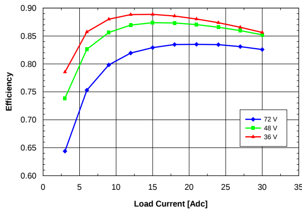
Fig. 1.5V.3: Efficiency vs. load current and input voltage for SQE48T30015 converter mounted vertically with air flowing from pin 3 to pin 1 at a rate of 300 LFM (1.5 m/s) and T_a = 25 °C.
