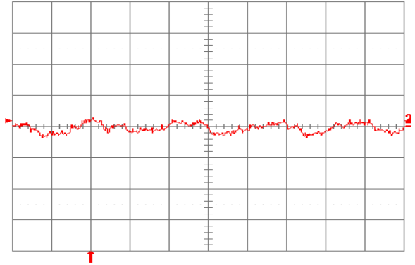
Fig. 3.3V.14: Input reflected-ripple current, i_s (10 mA/div.), measured through 10 \mu\text{H} at the source at full rated load current and V_{in} = 48 \text{ V} . Refer to Fig. 3.3V.12 for test setup. Time scale: 1 \mu\text{s}/\text{div.}
