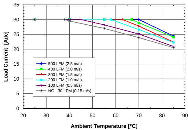
Fig. 2.5V.1: Available load current vs. ambient air temperature and airflow rates for SQE48T30025 converter mounted vertically with air flowing from pin 3 to pin 1, MOSFET temperature \leq 120 °C, V_{in} = 48 V.
