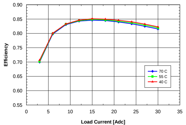
Fig. 1.2V.4: Efficiency vs. load current and ambient temperature for SQE48T30012 converter mounted vertically with V_{in} = 48 V and air flowing from pin 3 to pin 1 at a rate of 200 LFM (1.0 m/s).
