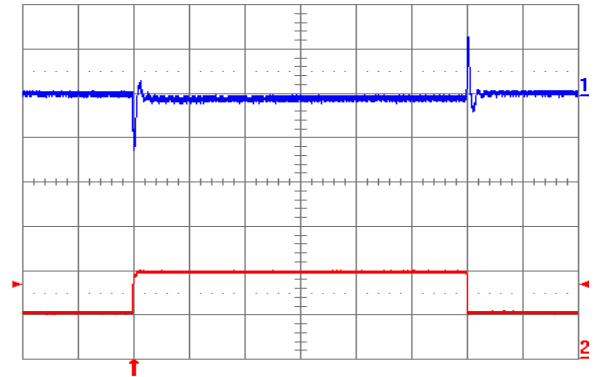
Fig. 1.2V.10: Output voltage response to load current step-change (10 A – 20 A – 10 A) at V_{in} = 48 V. Top trace: output voltage (100 mV/div.). Bottom trace: load current (10 A/div.). Current slew rate: 5 A/ \mu s. C_o = 470 \mu F POS + 1 \mu F ceramic. Time scale: 0.2 ms/div.
