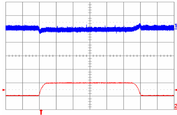
Fig. 3.3V.9: Output voltage response to load current step-change (10 A – 20 A – 10 A) at V_{in} = 48\text{ V} . Top trace: output voltage (100 mV/div.). Bottom trace: load current (10 A/div.). Current slew rate: 0.1 A/ \mu\text{s} . C_o = 1\text{ }\mu\text{F} ceramic. Time scale: 0.2 ms/div.
