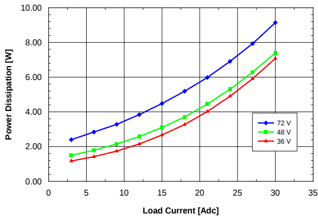
Fig. 1.2V.5: Power dissipation vs. load current and input voltage for SQE48T30012 converter mounted vertically with air flowing from pin 3 to pin 1 at a rate of 300 LFM (1.5 m/s) and T_a = 25^\circ\text{C} .
