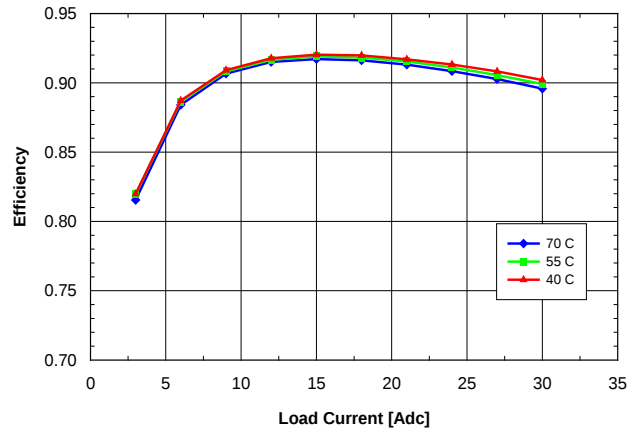
Fig. 3.3V.4: Efficiency vs. load current and ambient temperature for SQE48T30033 converter mounted vertically with V_{in} = 48 V and air flowing from pin 3 to pin 1 at a rate of 200 LFM (1.0 m/s).
