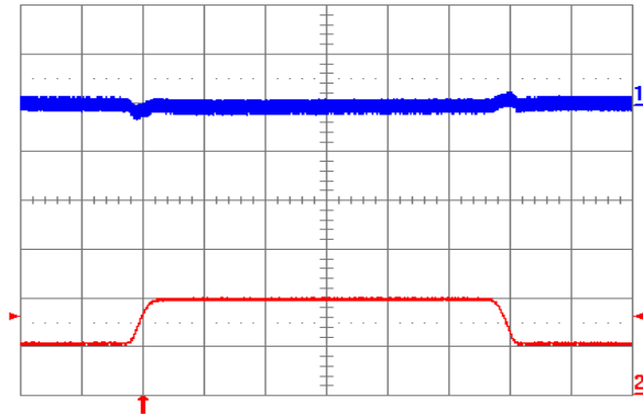
Fig. 1.5V.9: Output voltage response to load current step-change (10 A – 20 A – 10 A) at V_{in} = 48 V. Top trace: output voltage (100 mV/div.). Bottom trace: load current (10 A/div.). Current slew rate: 0.1 A/ \mu s. C_o = 1 \mu F ceramic. Time scale: 0.2 ms/div.
