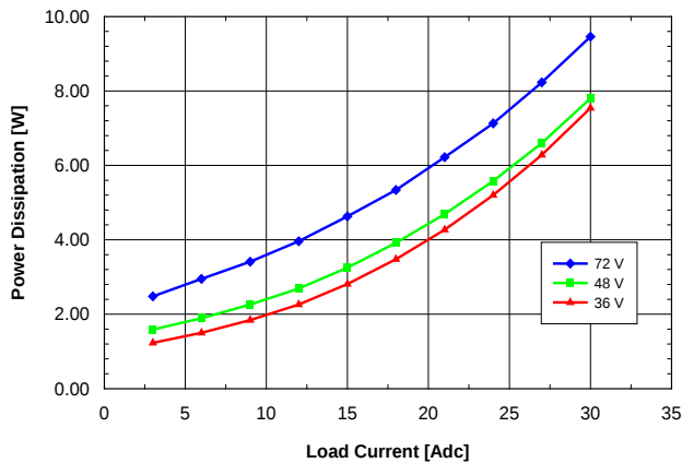
Fig. 1.5V.5: Power dissipation vs. load current and input voltage for SQE48T30015 converter mounted vertically with air flowing from pin 3 to pin 1 at a rate of 300 LFM (1.5 m/s) and T_a = 25^\circ\text{C} .
