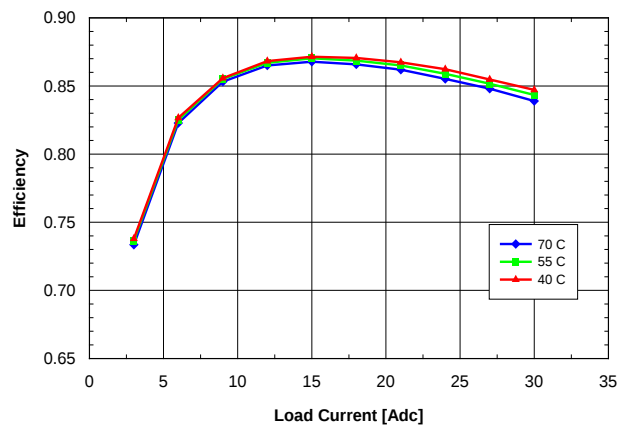
Fig. 1.5V.4: Efficiency vs. load current and ambient temperature for SQE48T30015 converter mounted vertically with V_{in} = 48 V and air flowing from pin 3 to pin 1 at a rate of 200 LFM (1.0 m/s).
