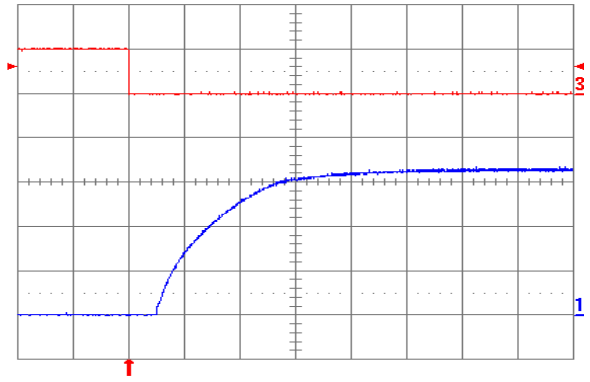
Fig. 3.3V.8: Turn-on transient at full rated load current (resistive) plus 10,000 \mu\text{F} at V_{in} = 48\text{ V} , triggered via ON/OFF pin. Top trace: ON/OFF signal (5 V/div.). Bottom trace: Output voltage (1 V/div.). Time scale: 1 ms/div.
