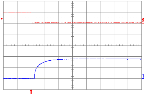
Fig. 1.8V.7: Turn-on transient at full rated load current (resistive) with no output capacitor at V_{in} = 48\text{ V} , triggered via ON/OFF pin. Top trace: ON/OFF signal (5 V/div.). Bottom trace: Output voltage (1 V/div.). Time scale: 2 ms/div.
