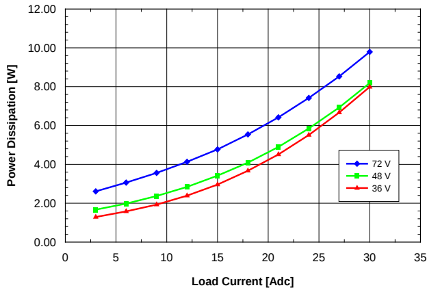
Fig. 1.8V.5: Power dissipation vs. load current and input voltage for SQE48T30018 converter mounted vertically with air flowing from pin 3 to pin 1 at a rate of 300 LFM (1.5 m/s) and T_a = 25^\circ\text{C} .
