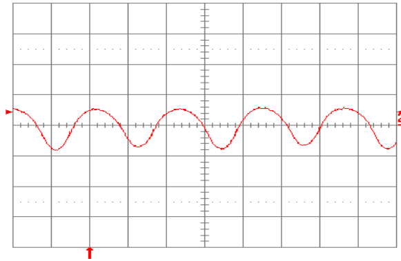
Fig. 1.5V.13: Input reflected ripple-current, i_r (100 mA/div.), measured at input terminals at full rated load current and V_{in} = 48 V. Refer to Fig. 1.5V.12 for test setup. Time scale: 1 \mu s/div.
