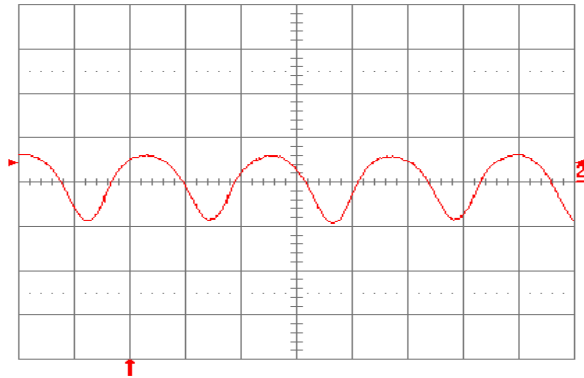
Fig. 1.2V.13: Input reflected ripple-current, i_c (100 mA/div.), measured at input terminals at full rated load current and V_{in} = 48 V. Refer to Fig. 1.2V.12 for test setup. Time scale: 1 \mu s/div.
