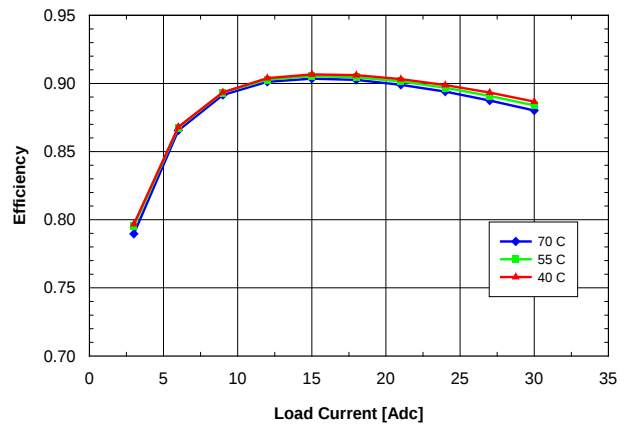
Fig. 2.5V.4: Efficiency vs. load current and ambient temperature for SQE48T30025 converter mounted vertically with V_{in} = 48 V and air flowing from pin 3 to pin 1 at a rate of 200 LFM (1.0 m/s).
