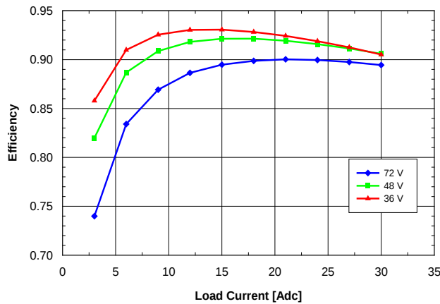
Fig. 3.3V.3: Efficiency vs. load current and input voltage for SQE48T30033 converter mounted vertically with air flowing from pin 3 to pin 1 at a rate of 300 LFM (1.5 m/s) and T_a = 25 °C.
