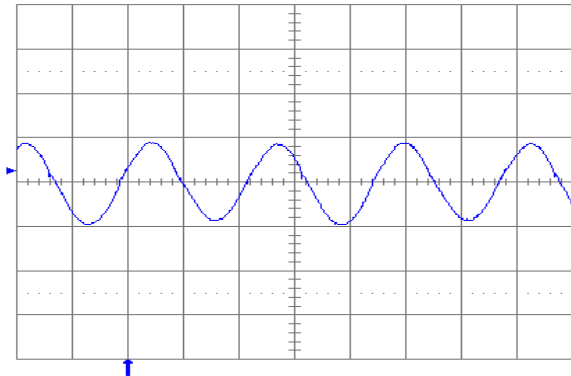
Fig. 3.3V.11: Output voltage ripple (20 mV/div.) at full rated load current into a resistive load with C_o = 10 \mu\text{F} tantalum + 1 \mu\text{F} ceramic and V_{in} = 48 \text{ V} . Time scale: 1 \mu\text{s}/\text{div.}
