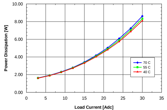
Fig. 1.5V.6: Power dissipation vs. load current and ambient temperature for SQE48T30015 converter mounted vertically with V_{in} = 48\text{ V} and air flowing from pin 3 to pin 1 at a rate of 200 LFM (1.0 m/s).
