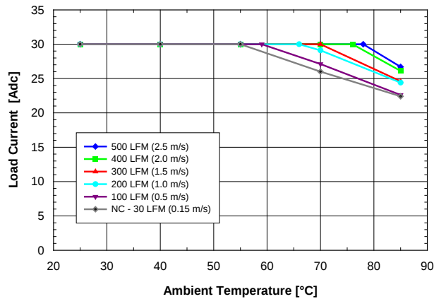
Fig. 1.8V.1: Available load current vs. ambient air temperature and airflow rates for SQE48T30018 converter mounted vertically with air flowing from pin 3 to pin 1, MOSFET temperature \leq 120 °C, V_{in} = 48 V.
