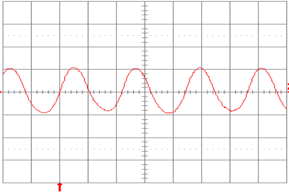
Fig. 3.3V.13: Input reflected-ripple current, i_c (50 mA/div.), measured at input terminals at full rated load current and V_{in} = 48 \text{ V} . Refer to Fig. 3.3V.12 for test setup. Time scale: 1 \mu\text{s}/\text{div.}
