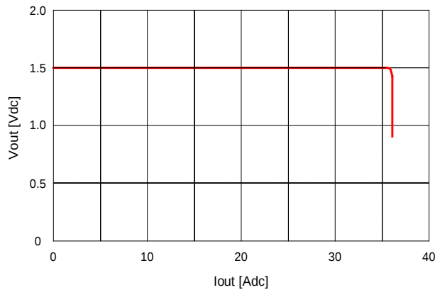
Fig. 1.5V.15: Output voltage vs. load current showing current limit point and converter shutdown point. Input voltage has almost no effect on current limit characteristic.
