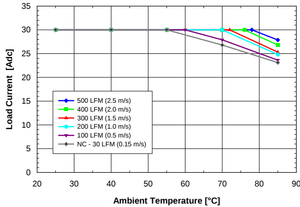
Fig. 1.5V.1: Available load current vs. ambient air temperature and airflow rates for SQE48T30015 converter mounted vertically with air flowing from pin 3 to pin 1, MOSFET temperature \leq 120 °C, V_{in} = 48 V.
