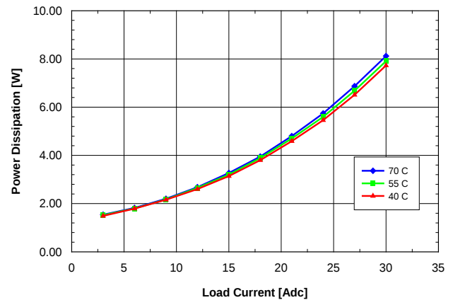
Fig. 1.2V.6: Power dissipation vs. load current and ambient temperature for SQE48T30012 converter mounted vertically with V_{in} = 48\text{ V} and air flowing from pin 3 to pin 1 at a rate of 200 LFM (1.0 m/s).
