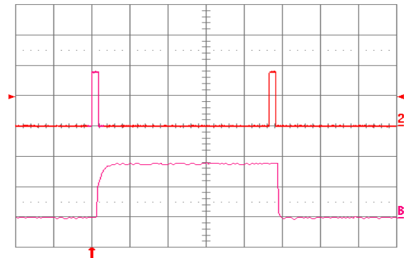
Fig. 1.5V.16: Load current (top trace, 20 A/div., 50 ms/div.) into a 10 m \Omega short circuit during restart, at V_{in} = 48 V. Bottom trace (20 A/div., 2 ms/div.) is an expansion of the on-time portion of the top trace.
