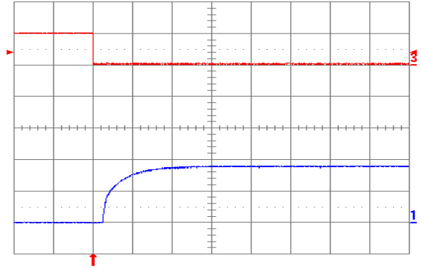
Fig. 1.8V.8: Turn-on transient at full rated load current (resistive) plus 10,000 \mu\text{F} at V_{in} = 48\text{ V} , triggered via ON/OFF pin. Top trace: ON/OFF signal (5 V/div.). Bottom trace: Output voltage (1 V/div.). Time scale: 2 ms/div.
