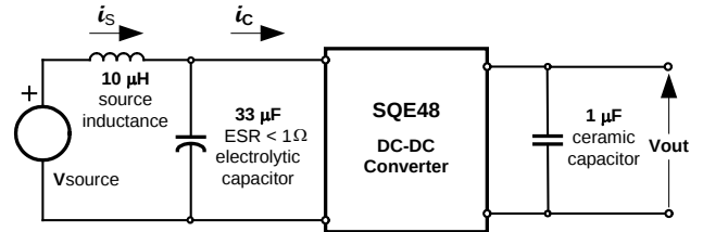
Fig. 3.3V.12: Test setup for measuring input reflected ripple currents, i_c and i_s .
