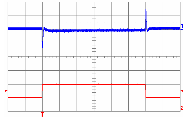
Fig. 3.3V.10: Output voltage response to load current step-change (10 A – 20 A – 10 A) at V_{in} = 48\text{ V} . Top trace: output voltage (100 mV/div.). Bottom trace: load current (10 A/div.). Current slew rate: 5 A/ \mu\text{s} . C_o = 470\text{ }\mu\text{F POS} + 1\text{ }\mu\text{F} ceramic. Time scale: 0.2 ms/div.
