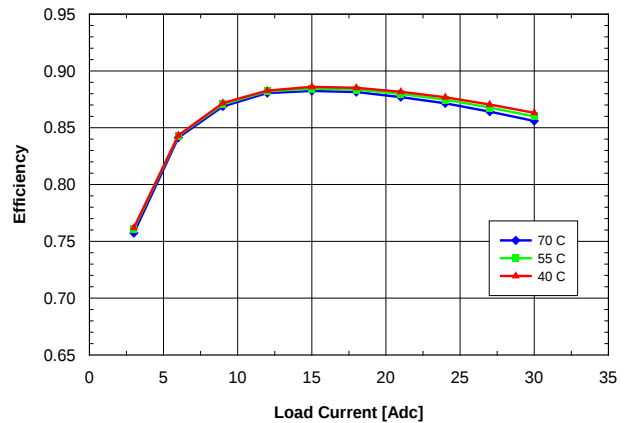
Fig. 1.8V.4: Efficiency vs. load current and ambient temperature for SQE48T30018 converter mounted vertically with V_{in} = 48 V and air flowing from pin 3 to pin 1 at a rate of 200 LFM (1.0 m/s).
