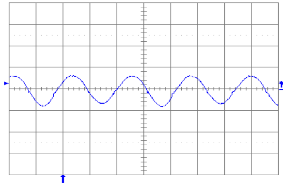
Fig. 2.5V.11: Output voltage ripple (20 mV/div.) at full rated load current into a resistive load with C_o = 10 \mu F tantalum + 1 \mu F ceramic and V_{in} = 48 V. Time scale: 1 \mu s/div.
