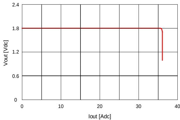
Fig. 1.8V.15: Output voltage vs. load current showing current limit point and converter shutdown point. Input voltage has almost no effect on current limit characteristic.
