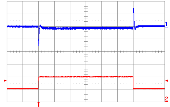
Fig. 1.8V.10: Output voltage response to load current step-change (10 A – 20 A – 10 A) at V_{in} = 48 V. Top trace: output voltage (100 mV/div.). Bottom trace: load current (10 A/div.). Current slew rate: 5 A/ \mu s. C_o = 470 \mu F POS + 1 \mu F ceramic. Time scale: 0.2 ms/div.
