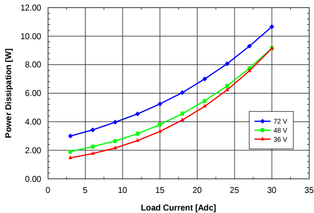
Fig. 2.5V.5: Power dissipation vs. load current and input voltage for SQE48T30025 converter mounted vertically with air flowing from pin 3 to pin 1 at a rate of 300 LFM (1.5 m/s) and T_a = 25^\circ\text{C} .
