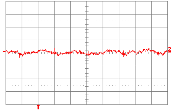
Fig. 1.2V.14: Input reflected-ripple current, i_s (10 mA/div.), measured through 10 \mu H at the source at full rated load current and V_{in} = 48 V. Refer to Fig. 1.2V.12 for test setup. Time scale: 1 \mu s/div.
