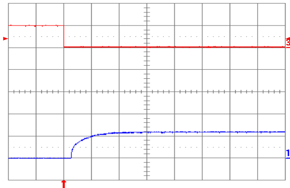
Fig. 1.2V.7: Turn-on transient at full rated load current (resistive) with no output capacitor at V_{in} = 48\text{ V} , triggered via ON/OFF pin. Top trace: ON/OFF signal (5 V/div.). Bottom trace: Output voltage (1 V/div.). Time scale: 2 ms/div.
