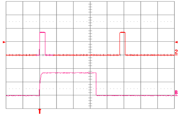
Fig. 1.2V.16: Load current (top trace, 20 A/div., 50 ms/div.) into a 10 m \Omega short circuit during restart, at V_{in} = 48 V. Bottom trace (20 A/div., 5 ms/div.) is an expansion of the on-time portion of the top trace.
