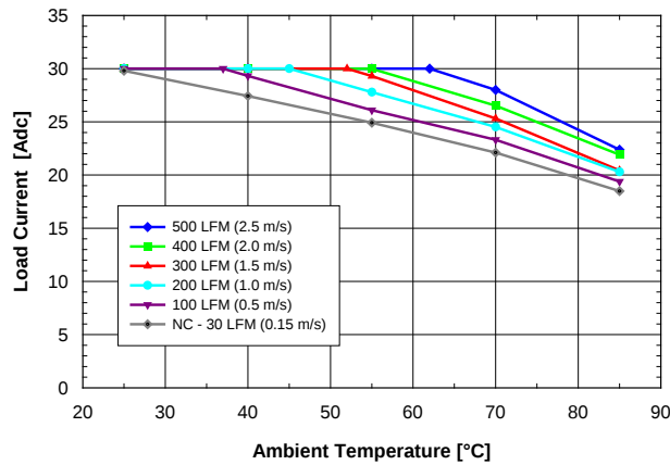
Fig. 3.3V.1: Available load current vs. ambient air temperature and airflow rates for SQE48T30033 converter mounted vertically with air flowing from pin 3 to pin 1, MOSFET temperature \leq 120 °C, V_{in} = 48 V.
