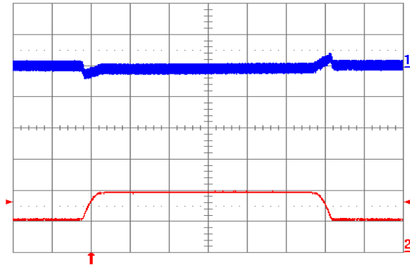
Fig. 2.5V.9: Output voltage response to load current step-change (10 A – 20 A – 10 A) at V_{in} = 48 V. Top trace: output voltage (100 mV/div.). Bottom trace: load current (10 A/div.). Current slew rate: 0.1 A/ \mu s. C_o = 1 \mu F ceramic. Time scale: 0.2 ms/div.
