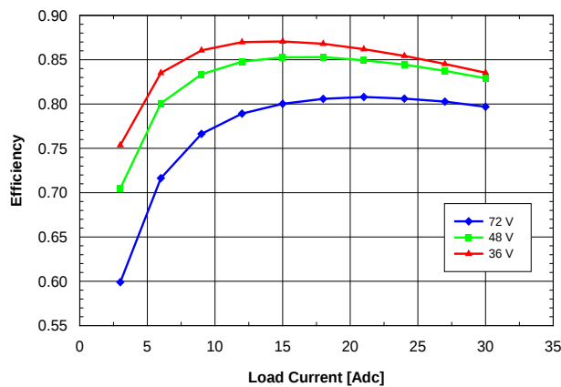
Fig. 1.2V.3: Efficiency vs. load current and input voltage for SQE48T30012 converter mounted vertically with air flowing from pin 3 to pin 1 at a rate of 300 LFM (1.5 m/s) and T_a = 25 °C.
