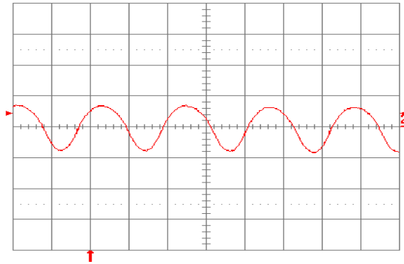
Fig. 1.8V.13: Input reflected-ripple current, i_e (100 mA/div.), measured at input terminals at full rated load current and V_{in} = 48 V. Refer to Fig. 1.8V.12 for test setup. Time scale: 1 \mu s/div.
