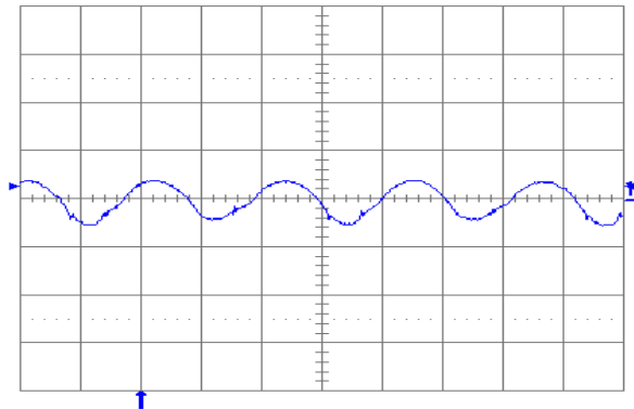
Fig. 1.2V.11: Output voltage ripple (20 mV/div.) at full rated load current into a resistive load with C_o = 10 \mu F tantalum + 1 \mu F ceramic and V_{in} = 48 V. Time scale: 1 \mu s/div.
