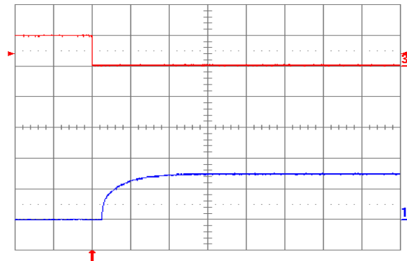
Fig. 1.5V.7: Turn-on transient at full rated load current (resistive) with no output capacitor at V_{in} = 48\text{ V} , triggered via ON/OFF pin. Top trace: ON/OFF signal (5 V/div.). Bottom trace: Output voltage (1 V/div.). Time scale: 2 ms/div.
