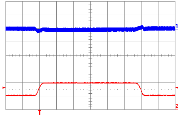
Fig. 1.8V.9: Output voltage response to load current step-change (10 A – 20 A – 10 A) at V_{in} = 48 V. Top trace: output voltage (100 mV/div.). Bottom trace: load current (10 A/div.). Current slew rate: 0.1 A/ \mu s. C_o = 1 \mu F ceramic. Time scale: 0.2 ms/div.
