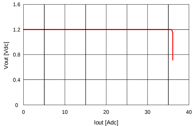
Fig. 1.2V.15: Output voltage vs. load current showing current limit point and converter shutdown point. Input voltage has almost no effect on current limit characteristic.
