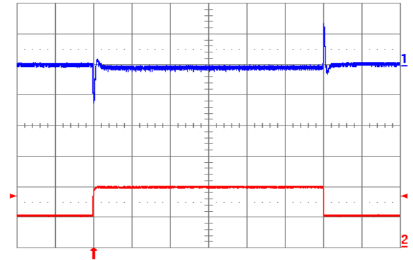
Fig. 1.5V.10: Output voltage response to load current step-change (10 A – 20 A – 10 A) at V_{in} = 48 V. Top trace: output voltage (100 mV/div.). Bottom trace: load current (10 A/div.). Current slew rate: 5A/ \mu s. C_o = 470 \mu F POS + 1 \mu F ceramic. Time scale: 0.2 ms/div.
