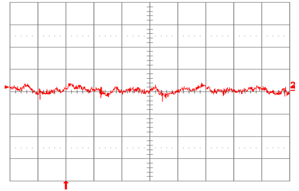
Fig. 1.8V.14: Input reflected-ripple current, i_s (10 mA/div.), measured through 10 \mu H at the source at full rated load current and V_{in} = 48 V. Refer to Fig. 1.8V.12 for test setup. Time scale: 1 \mu s/div.
