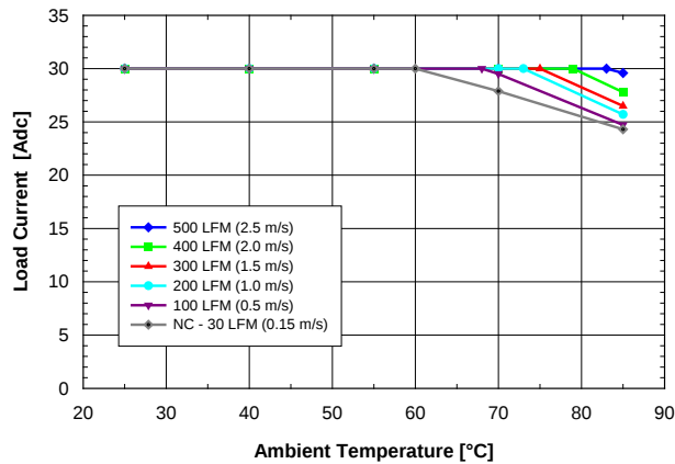
Fig. 1.2V.1: Available load current vs. ambient air temperature and airflow rates for SQE48T30012 converter mounted vertically with air flowing from pin 3 to pin 1, MOSFET temperature \leq 120 °C, V_{in} = 48 V.
