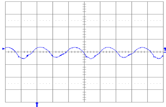
Fig. 1.5V.11: Output voltage ripple (20 mV/div.) at full rated load current into a resistive load with C_o = 10 \mu F tantalum + 1 \mu F ceramic and V_{in} = 48 V. Time scale: 1 \mu s/div.
