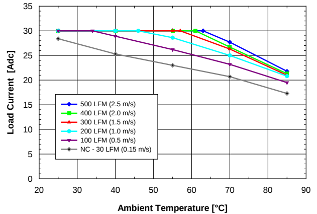
Fig. 3.3V.2: Available load current vs. ambient air temperature and airflow rates for SQE48T30033 converter mounted horizontally with air flowing from pin 3 to pin 1, MOSFET temperature \leq 120 °C, V_{in} = 48 V.
