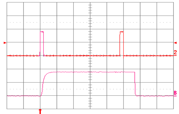
Fig. 1.8V.16: Load current (top trace, 20 A/div., 50 ms/div.) into a 10 m \Omega short circuit during restart, at V_{in} = 48 V. Bottom trace (20 A/div., 2 ms/div.) is an expansion of the on-time portion of the top trace.
