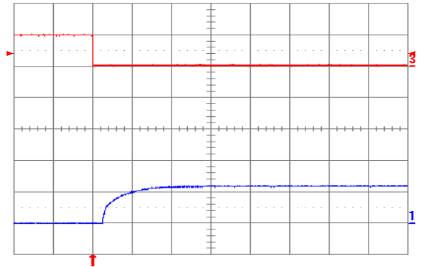
Fig. 1.2V.8: Turn-on transient at full rated load current (resistive) plus 10,000 \mu\text{F} at V_{in} = 48\text{ V} , triggered via ON/OFF pin. Top trace: ON/OFF signal (5 V/div.). Bottom trace: Output voltage (1 V/div.). Time scale: 2 ms/div.
