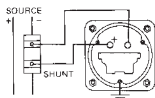
With external shunt
