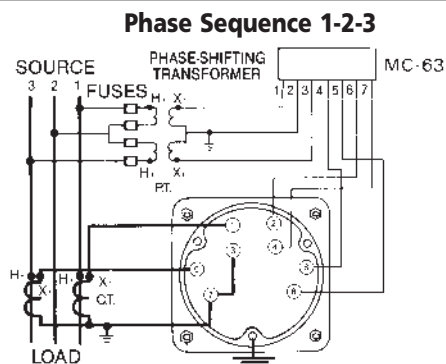
Connections for 3 wire, 3 phase varmeter with phase shifting transformer. (Balanced V) 10332-xxxx7xxx 103772xxxx7xxx
