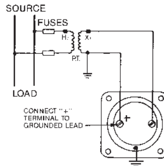
Frequency Meter with potential transformer 103372xxxx
