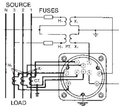
Four-wire, three-phase wattmeter with current transformer and potential transformer (Balanced V) 10325-xxxx7xxx 103732xxxx7xxx
