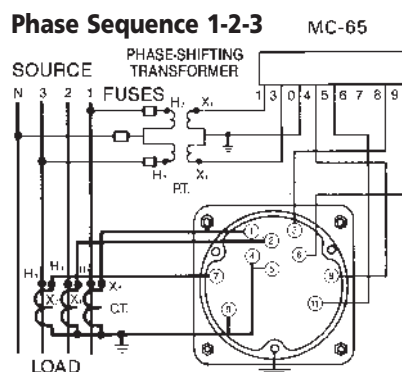
Connections for 4 wire, 3 phase varmeter with phase shifting transformer. (Balanced V) 10334-xxxx7xxx 103792xxxx7xxx
