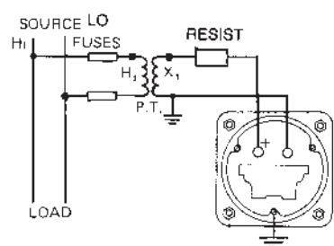
With potential transformer & external resistor
