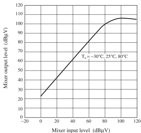
Mixer characteristic
