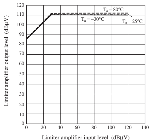
Limiter amplifier characteristics
