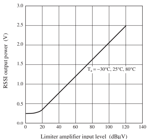
RSSI characteristic
