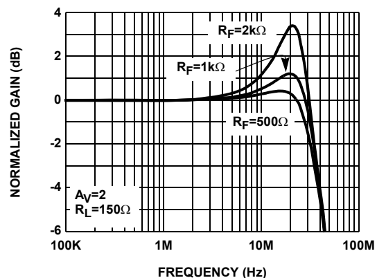
FIGURE 5. FREQUENCY RESPONSE FOR VARIOUS R_F
