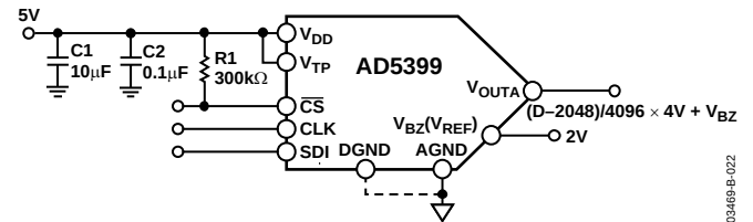
Figure 24. Disable \overline{\text{CS}} for Random Logic Mode
