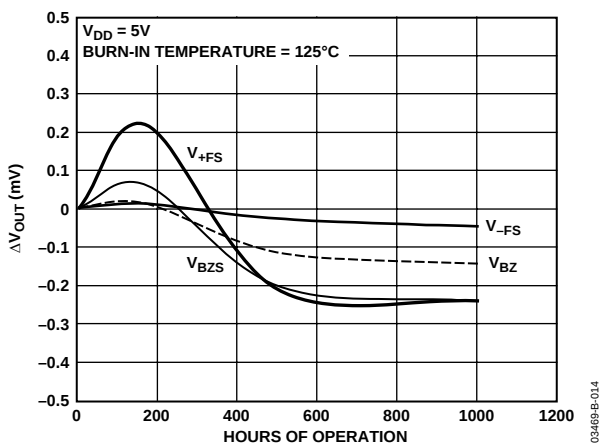
Figure 14. Long-Term Drift
