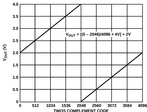
Figure 2. Output vs. Twos Complement Code
