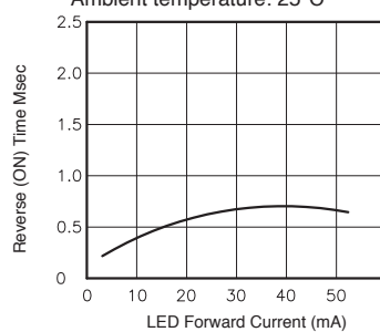
Fig.11 LED forward current vs. Reverse (ON) time Across terminals 5,7 and 6,8 pin; Load voltage: 400V (DC); Continuous load current: 130mA (DC); Ambient temperature: 25°C
