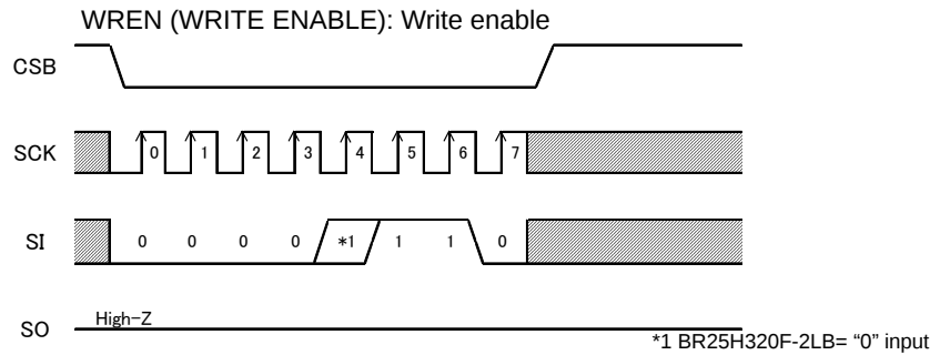
Figure 35. Write enable command
