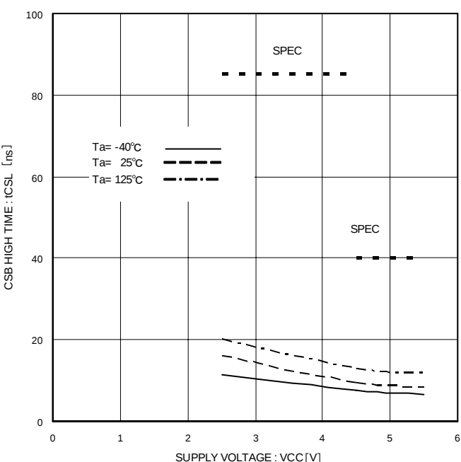
Figure 20. CSB High Time t_{CSL}
