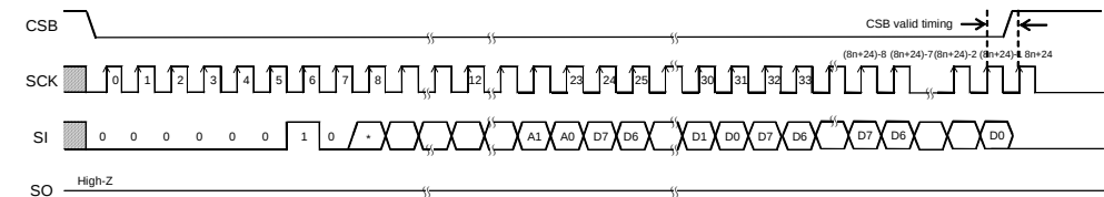
Figure 39. N Byte page write command
