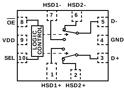
ISL54222A (10 LD 1.8X1.4 \mu TQFN) TOP VIEW
