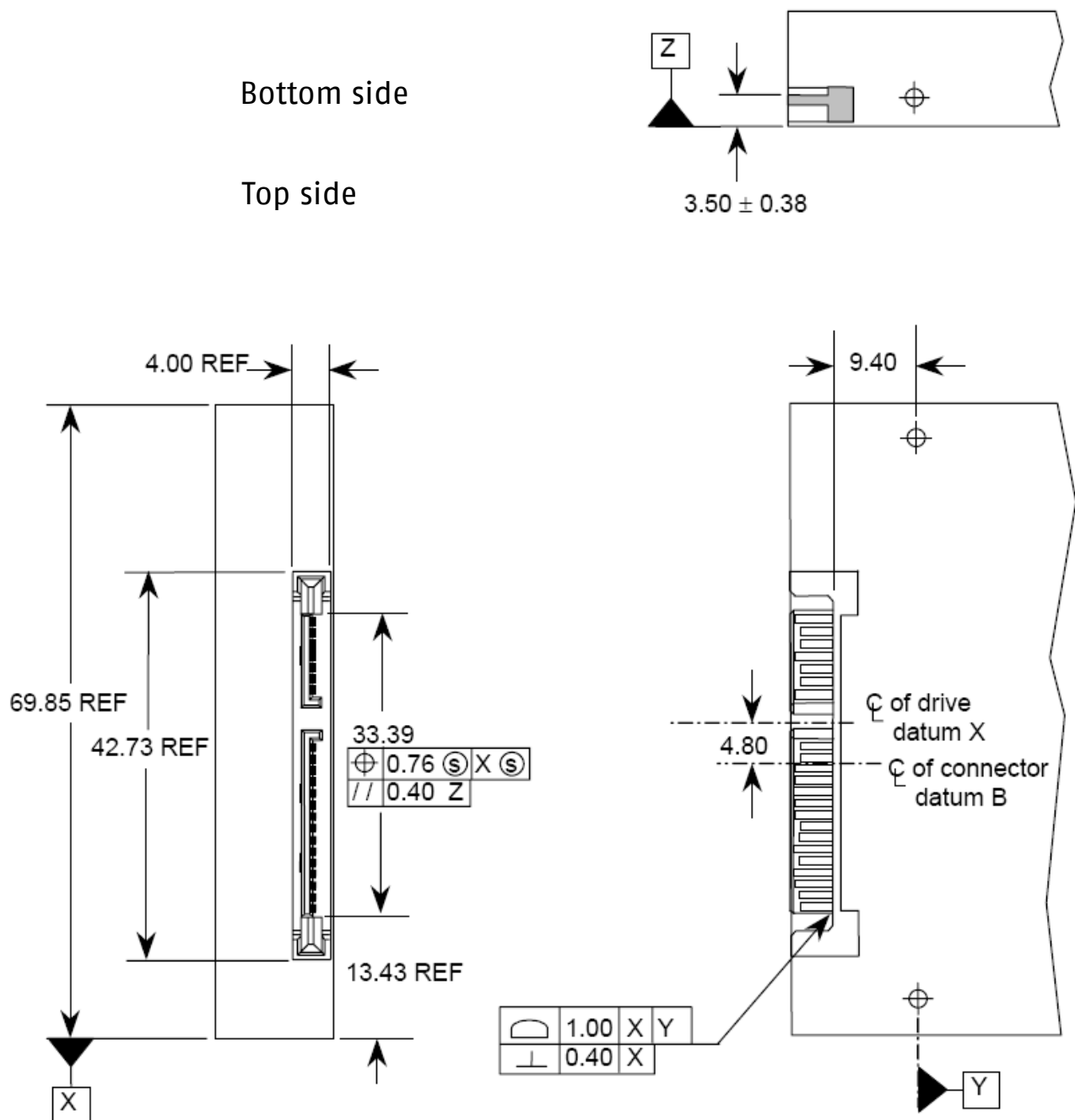
Figure 2: Connector location
