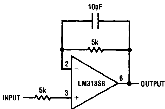
Voltage Follower
