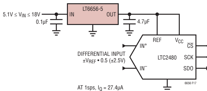
Figure 17. Low Power ADC Reference
