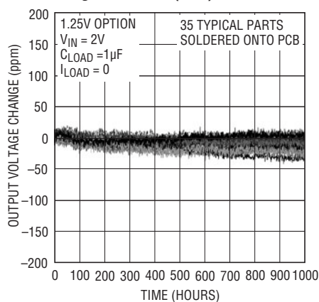
Long-Term Drift (LS8)
