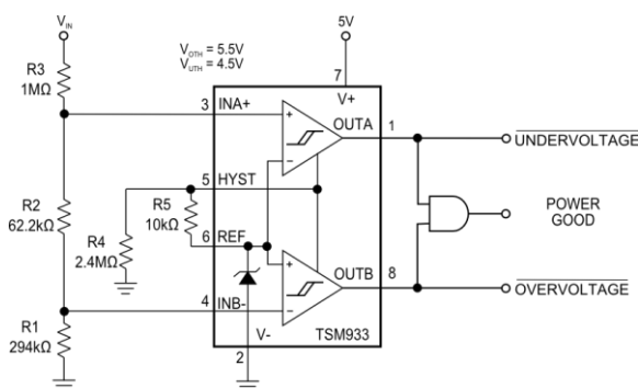
Figure 5. Window Detector
