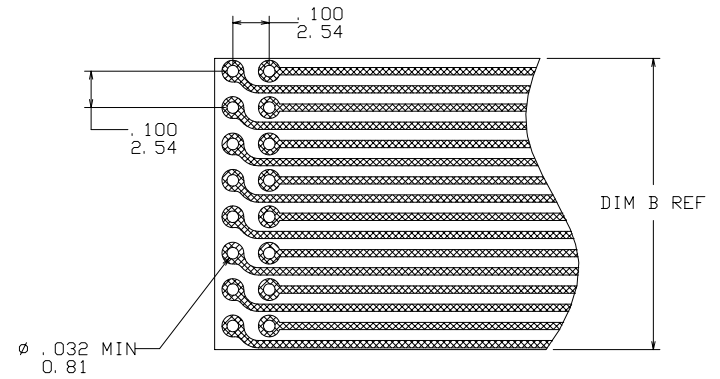
CABLE HOLE PATTERN
