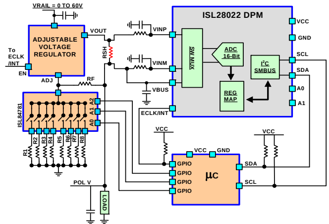
FIGURE 48. ADJUSTABLE POINT OF LOAD MONITORING DESIGN IDEA
