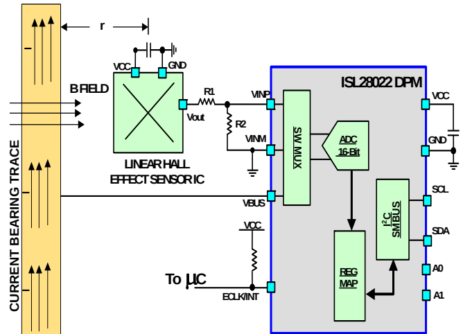
FIGURE 53. A SIMPLIFIED CIRCUIT DIAGRAM OF REMOTELY MEASURING CURRENT THROUGH A TRACE
