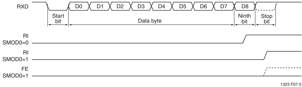
FIGURE 6-3: UART Timings in Modes 2 and 3
