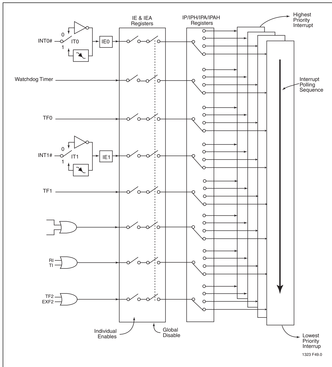
FIGURE 9-2: Interrupt Sequence
