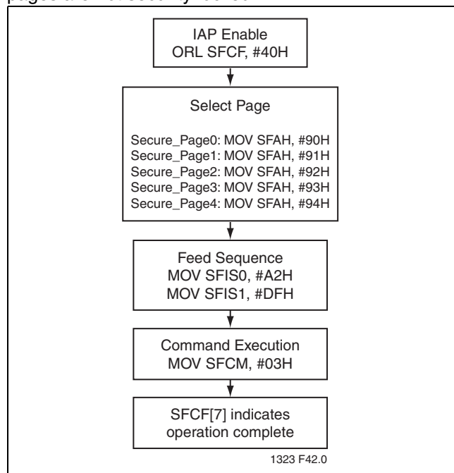
FIGURE 4-6: Secure-Page0-4
