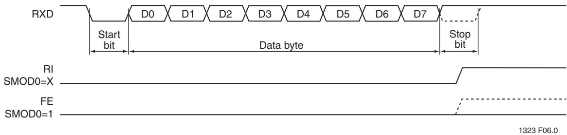
FIGURE 6-2: UART Timings in Mode 1
