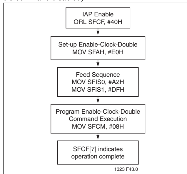
FIGURE 4-7: Enable-Clock-Double
