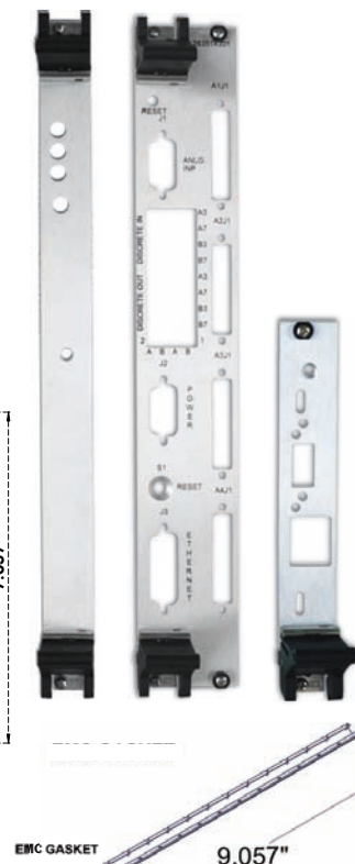
VECTOR P/N: 93400156 MATERIAL: STEEL WITH BRIGHT NICKEL FINISH
