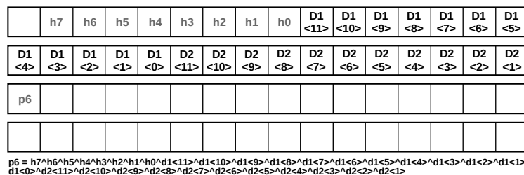
Figure 75. p6 Bit for 64-Bit Packet: 12-Bit Case
