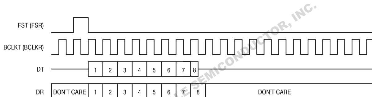
Figure 2b. Short Frame Sync (Transmit and Receive Have Individual Clocking)
