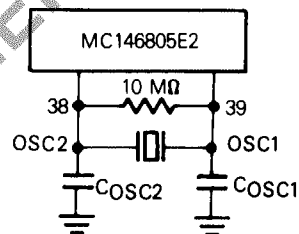
Crystal Oscillator Connections
