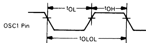
Oscillator Waveform
