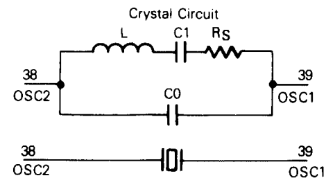
Crystal Circuit
