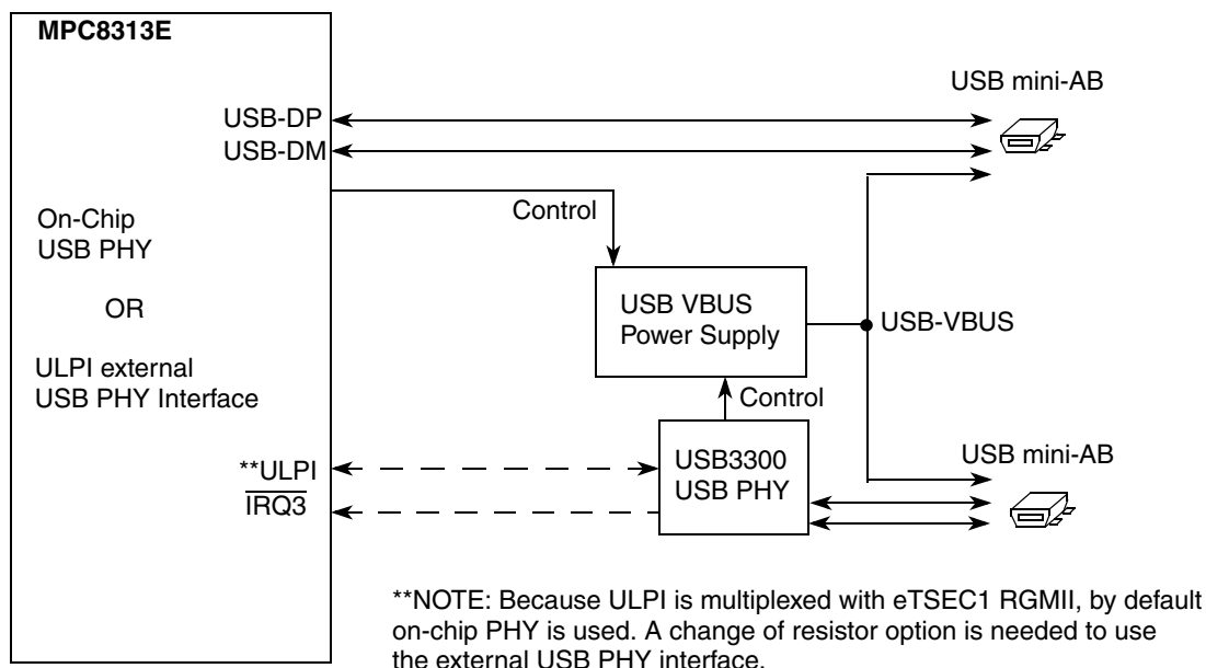
Figure 13. USB Connections
