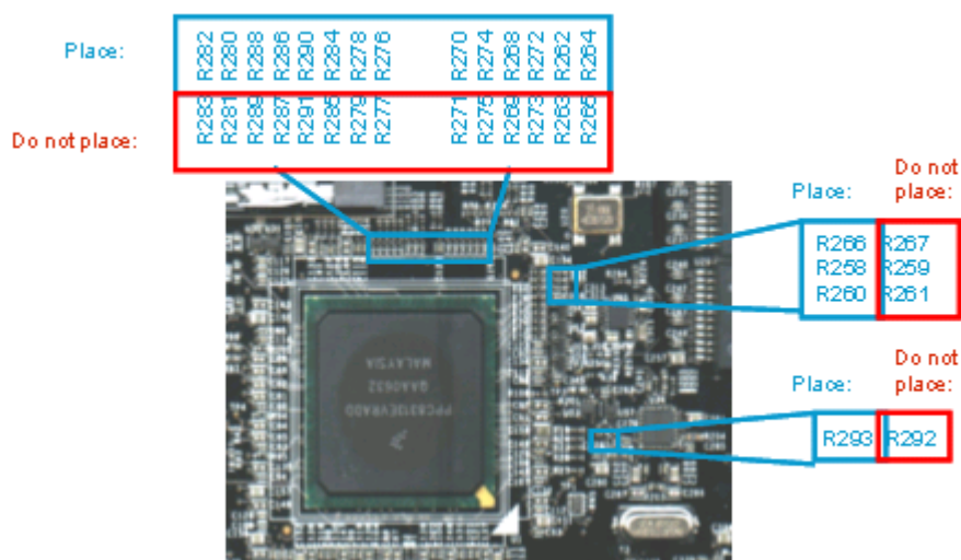
Figure 35. Setup 4 Resistor Options for REVA1
