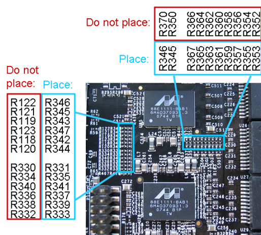
Figure 38. Setup 3 Resistor Options for REVC
