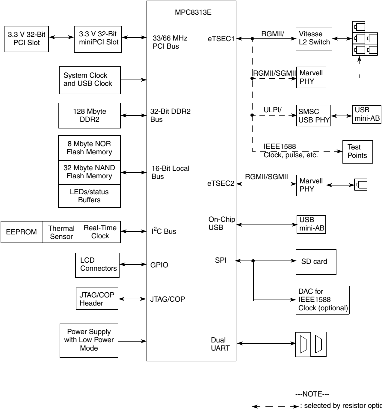
Figure 1. MPC8313E RDB Block Diagram
