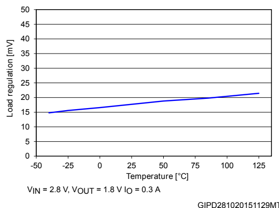
Figure 7. Load regulation vs. temperature
