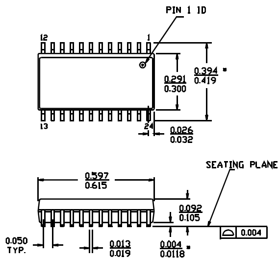
24-Lead (300-Mil) Molded SOIC S13
