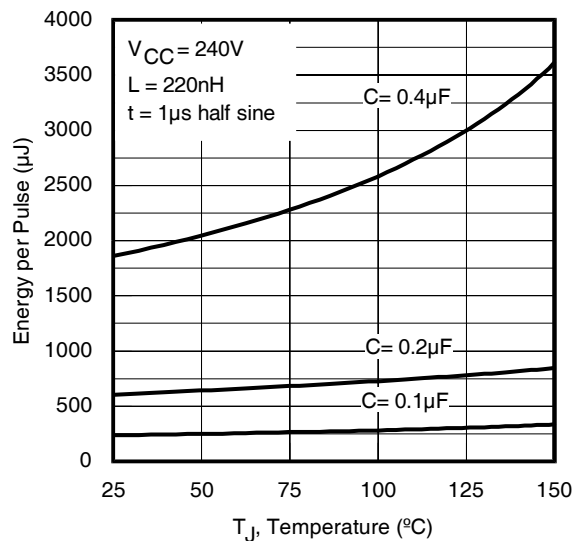
Fig 11. E_{\text{PULSE}} vs. Temperature
