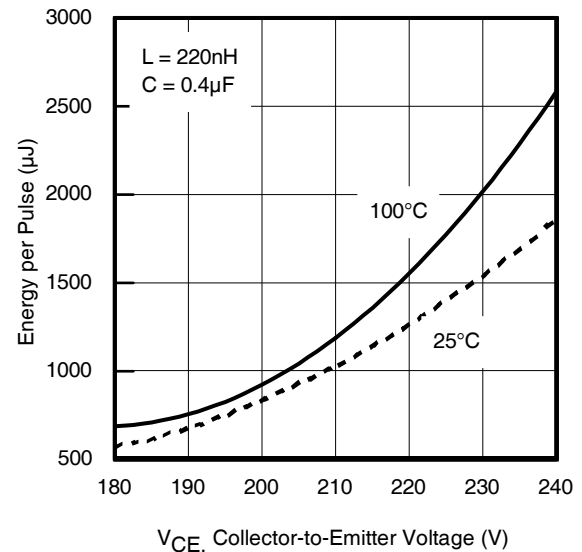
Fig 10. Typical E_{\text{PULSE}} vs. Collector-to-Emitter Voltage
