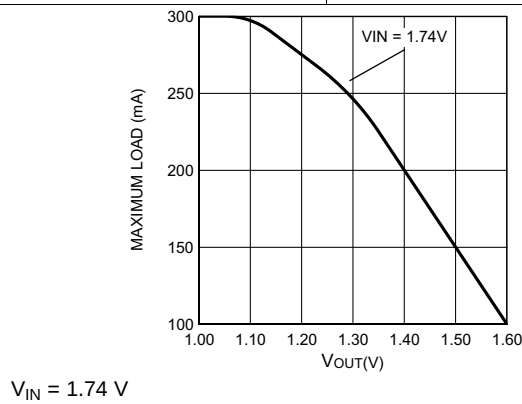
Figure 9. LDO Maximum Load
