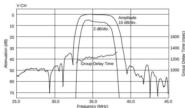
Frequency Characteristics(Pictuer-ch)
