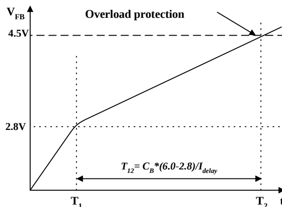
Figure 8. Overload Protection
