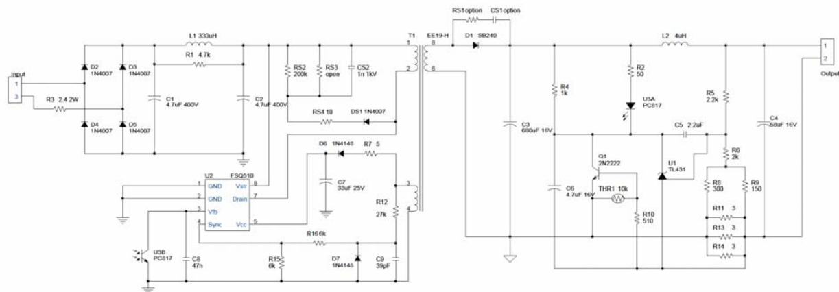
Figure 13. FSQ510 Schematic
