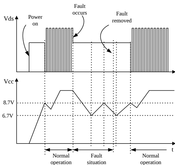
Figure 7. Auto Restart Protection Waveforms
